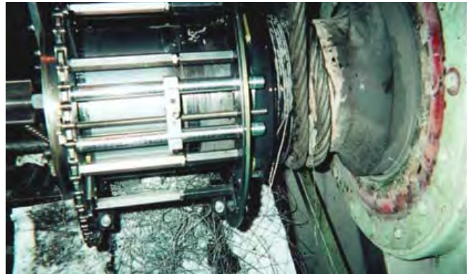
A 300mm Ø Fanshaft Journal During Machining
